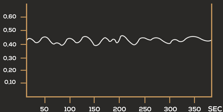
Friction coefficient of Steinhof CV Brake Pads
